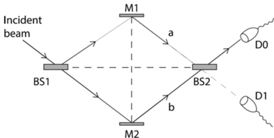
Figure 4 - Mach-Zehnder interferometer
