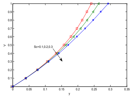
Fig6. Velocity profile for different values of S
