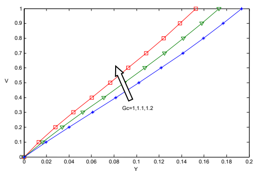
Fig3. Velocity profile for different values of Gc
